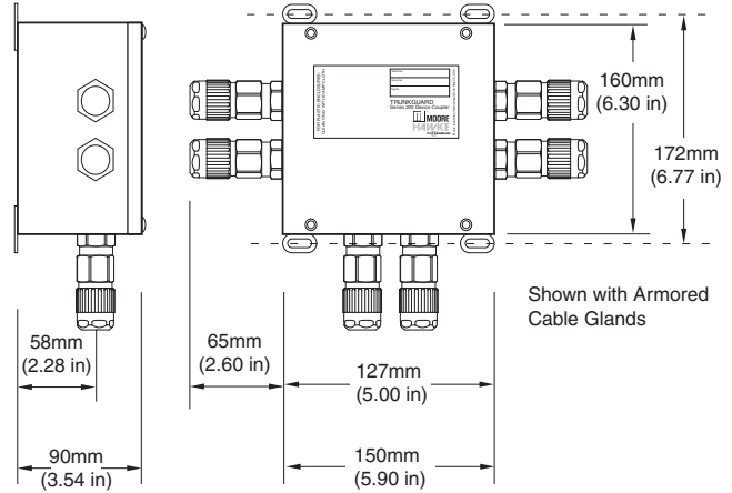
Figure 5. Electro-Polished Stainless Steel 316 Enclosure Installation Dimensions for 4-Spur (TG224) Models.
