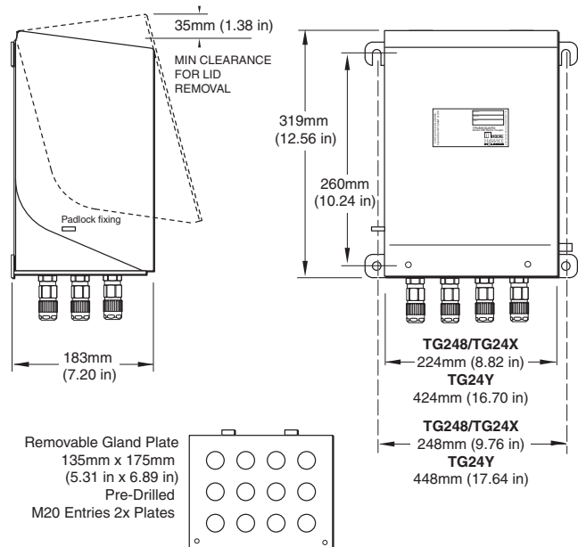
Figure 7. Stainless Steel 316 with E-Z Vertically Removable Lid and Bottom Entry Cable Gland Plate Installation Dimensions for 8-Spur (TG248), 10-Spur (TG24X), 12-Spur (TG2W) and 20-Spur (TG24Y) Models.
