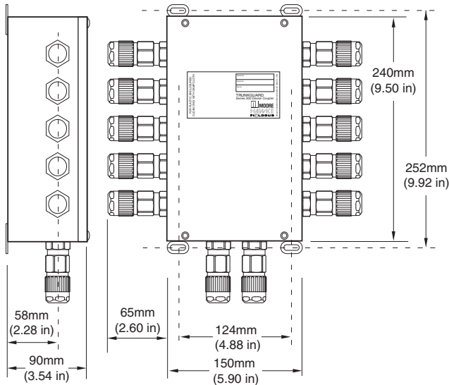
Figure 6. Electro-Polished Stainless Steel 316 Enclosure Installation Dimensions for 8- (TG228) and 10-Spur (TG22X) Models.
