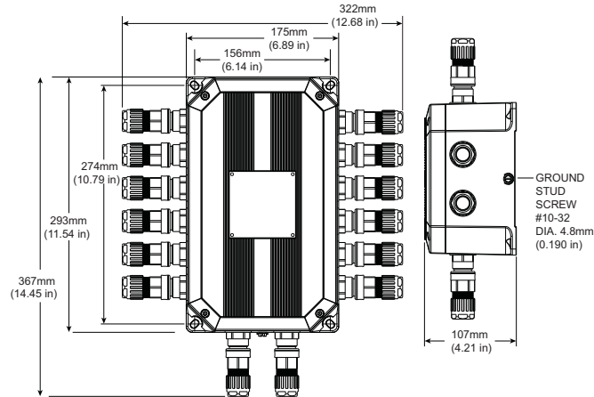
Figure 4. Standard Aluminum Enclosure Installation Dimensions for 4-Spur (TG25/64), 8-Spur (TG25/68), 10-Spur (TG25/6X) and 12-Spur (TG25/6W) Models.
