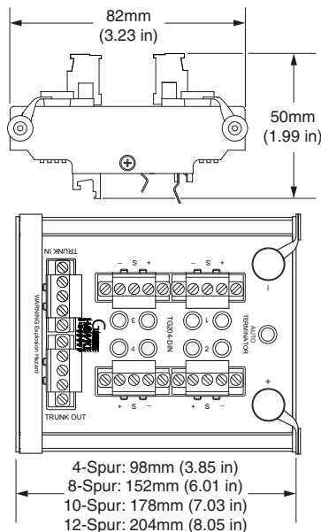
Figure 2. DIN-Rail Mounting Installation Dimensions (Base Units).
