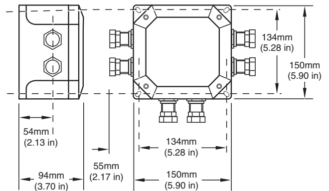
Figure 3. GRP (Glass Reinforced Polyester) Enclosure Installation Dimensions for TG234 (4-Spur) Models.
